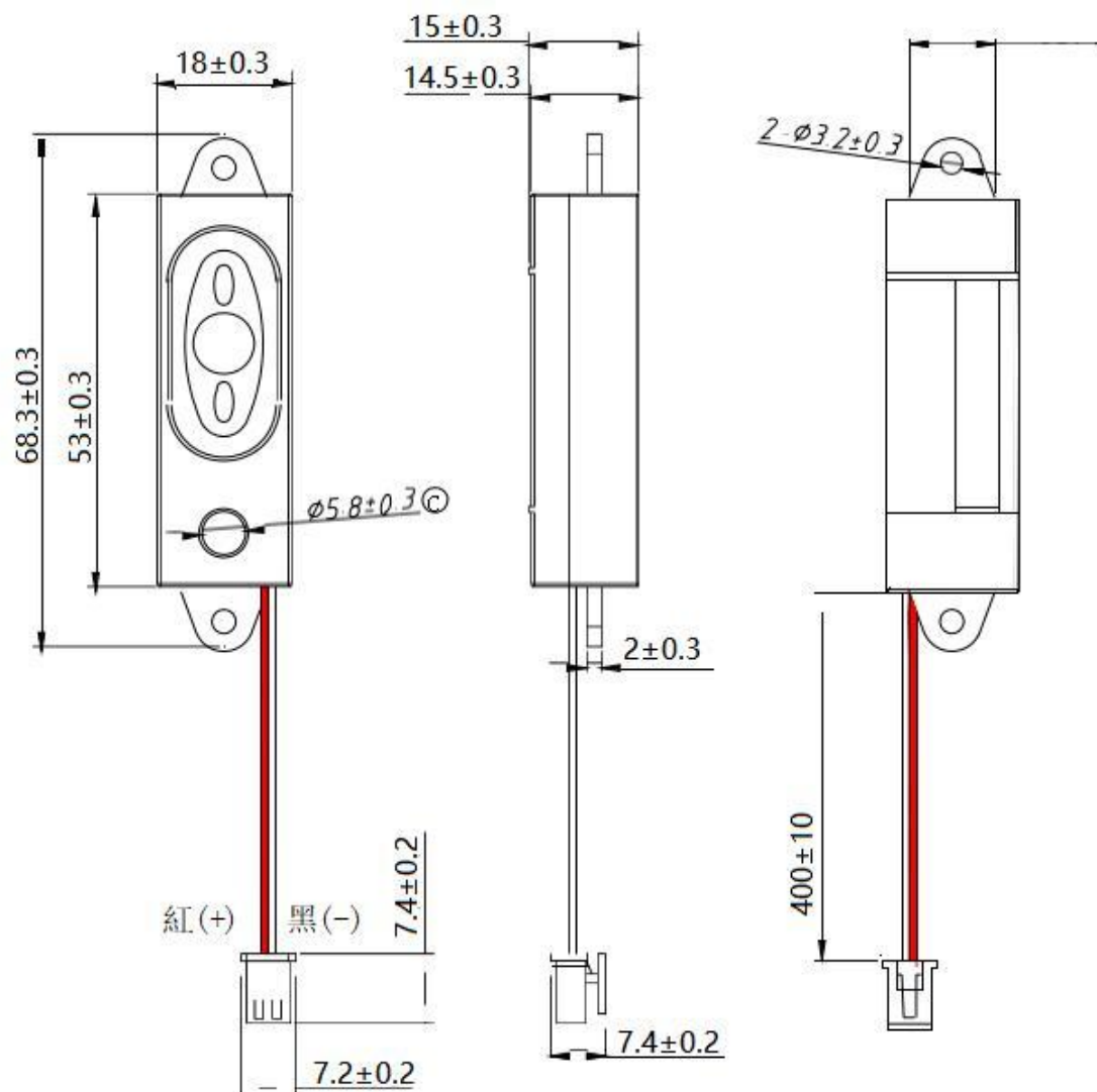
HOUSING:SMH250-02,Pitch2.5,黑色(端子鍍錫) WIRE:UL1571 28AWG紅黑并線,OD=0.88±0.05
